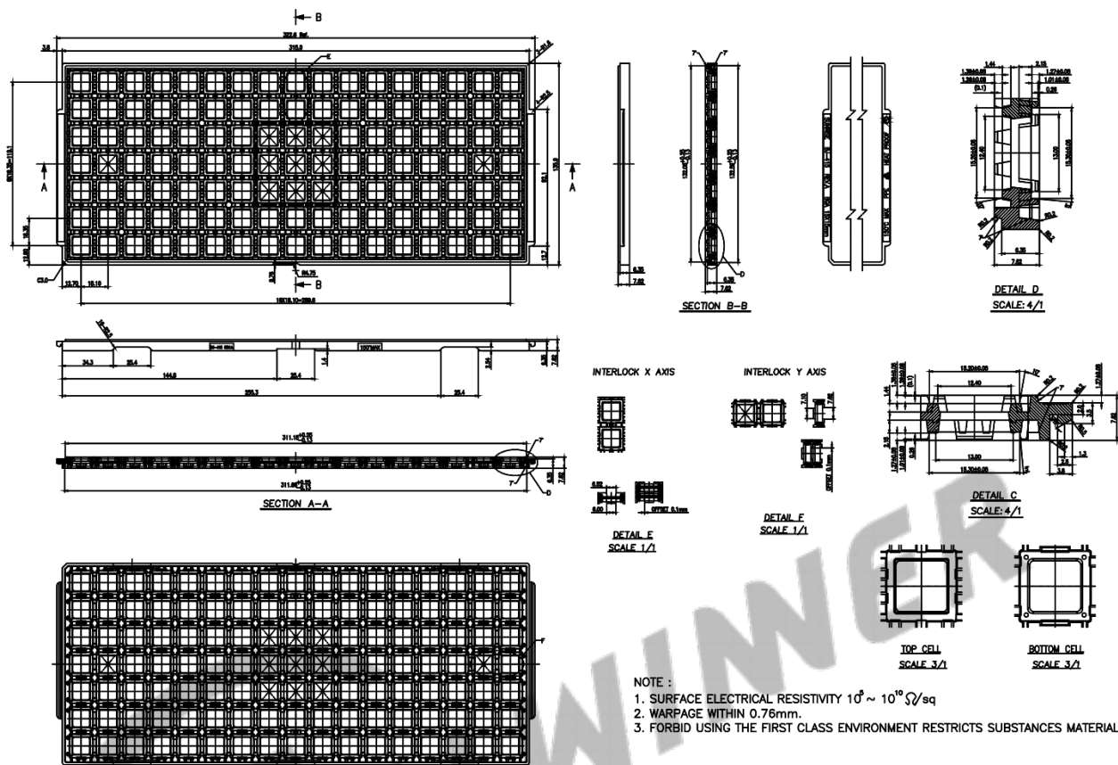
Figure 8-1 Tray Dimension Drawing
