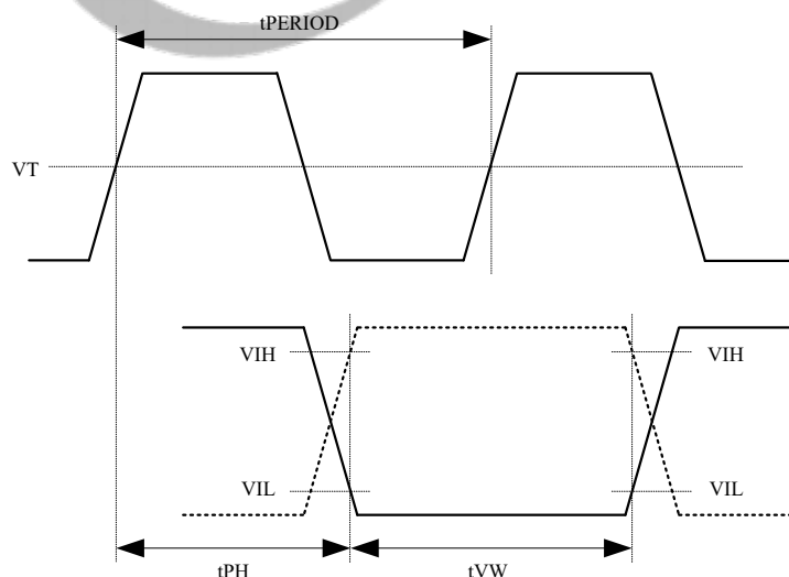
Figure 5-17 SMHC HS200/SDR104 Mode Input Timing Diagram
