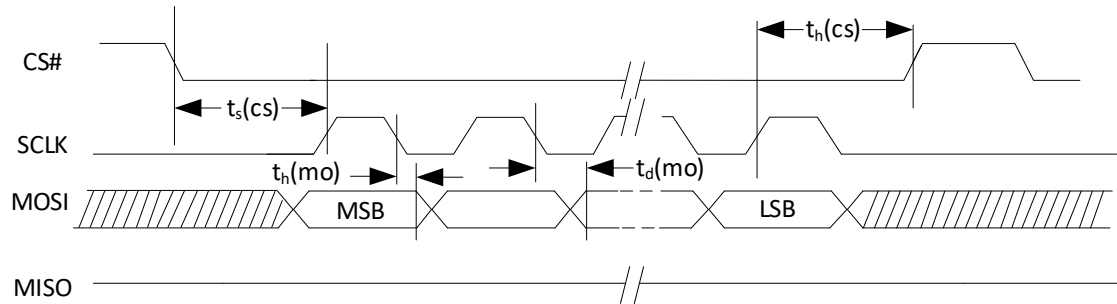
Figure 5-29 SPI Writing Timing
